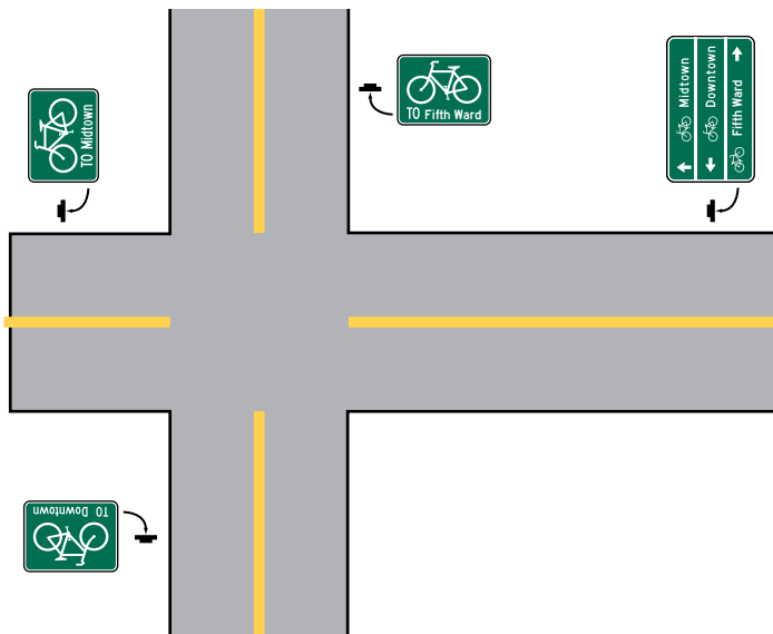
Figure 4.19 Typical sign placement at an intersection.
