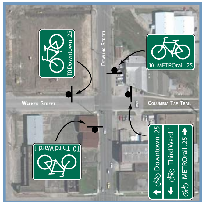
Example of typical sign placement at an intersection using standard MUTCD signage
