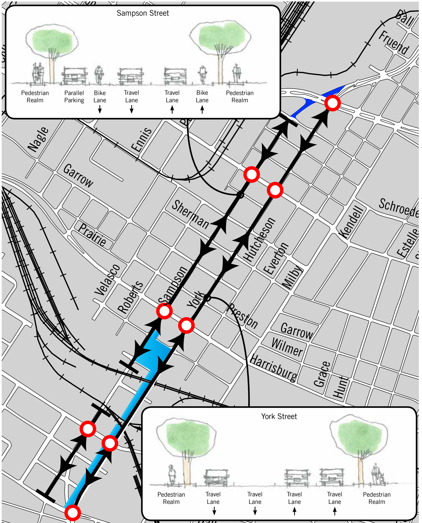
Figure 4.8 Potential Sampson Street and York Street Two-way Operation
