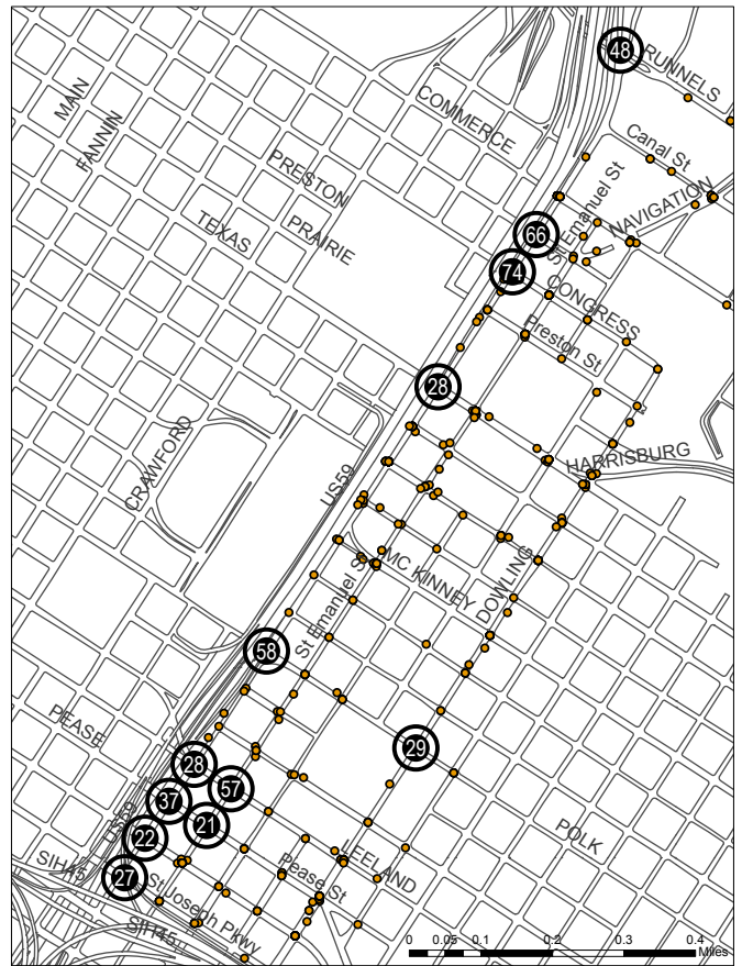
Figure 4.10 Intersections with Greater than 20 Crashes 2006-2010
