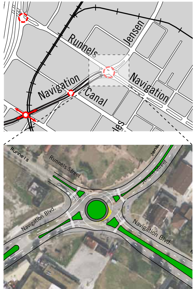
Figure 4.2 Conceptual Plan for Navigation Boulevard at Jensen / Runnels Roundabout
