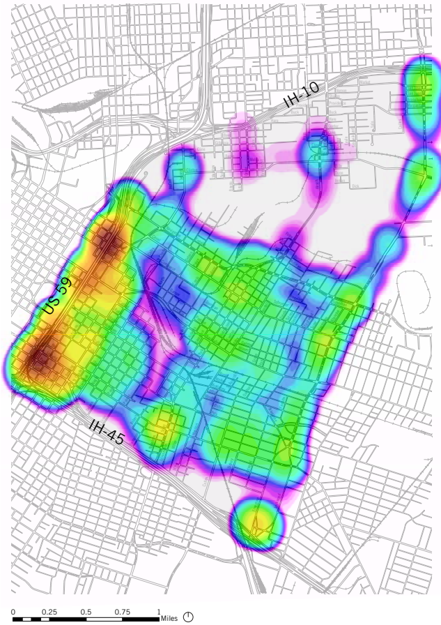
Figure 2.17 Crash Density - All Crashes
