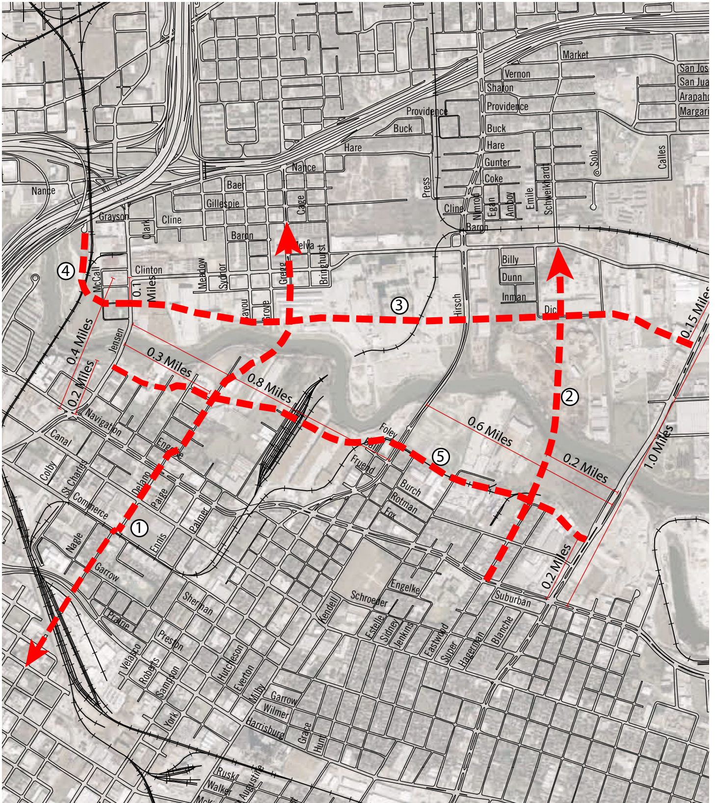
Figure 4.21 Potential Collector Roadways
